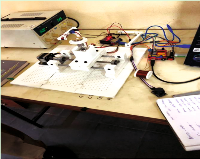
Test Rig installed by IAAHP KITSW Team at KITSW to study the properties of ring Magnet used in Centrimag motor
